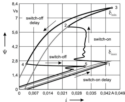
Figure 2: Operation cycle (activation/deactivation operation) of an electromagnet with cycle direction
