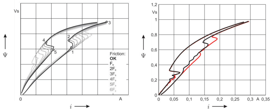
Figure 9 and 10: Left: Endurance testing with several million cycles and increased friction due to wear. Right: measurement under pressure shows influence of counter forces
