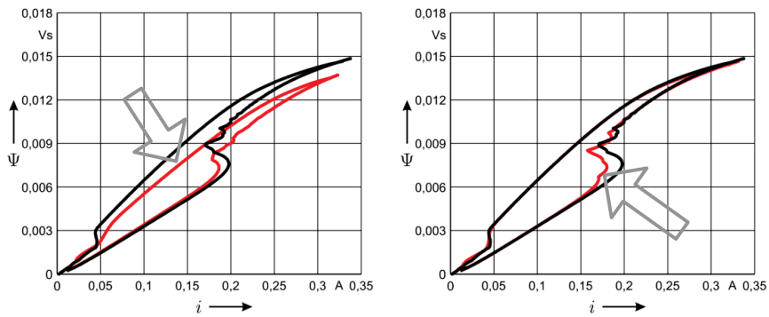
Figure 7 and 8: Left: contamination on the upper armature side. Right: broken leg of the membrane spring
