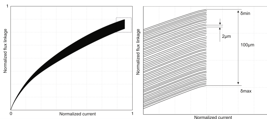
Figure 3 und 4: Left: \Psi(i, \delta) family of characteristics of a solenoid with fix armature positions in 2 μm steps. Right: Detail of the \Psi(i, \delta) characteristics
