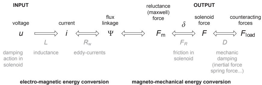
Figure 1: Energy conversion in solenoid
