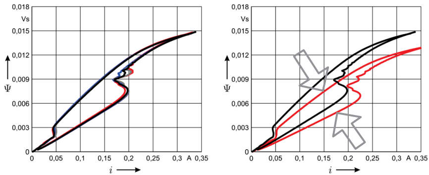
Figure 5 and 6: Left: four good magnetic valves without errors. Small deviations through the production process are visible. Right: short-circuit between turns of the coil with 10% reduced active winding
