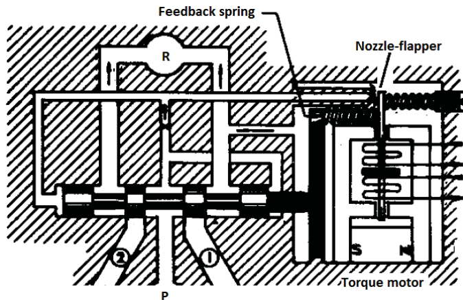
(b) Cadillac Gage FC-2
