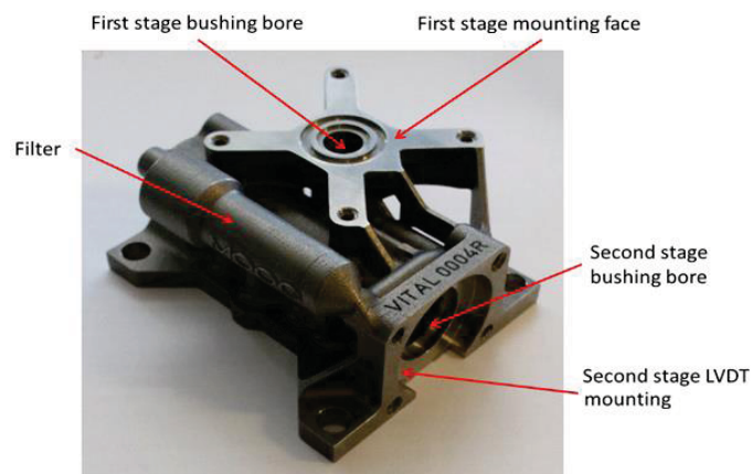
Figure 16: Detail of AM valve body
