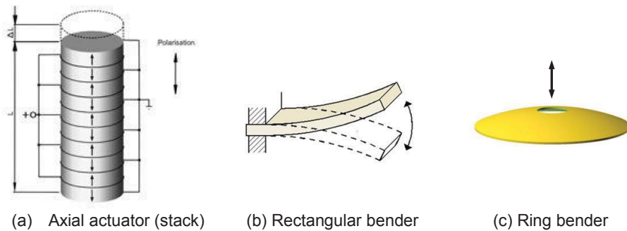
Figure 7. Piezoelectric actuation
